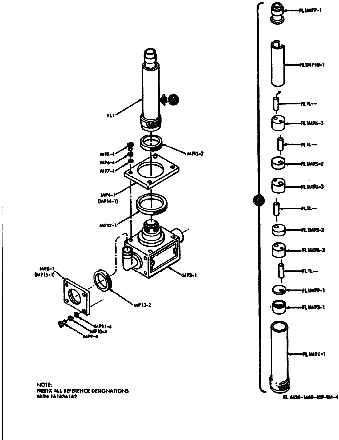
Figure 5. RF Coupler Assembly
