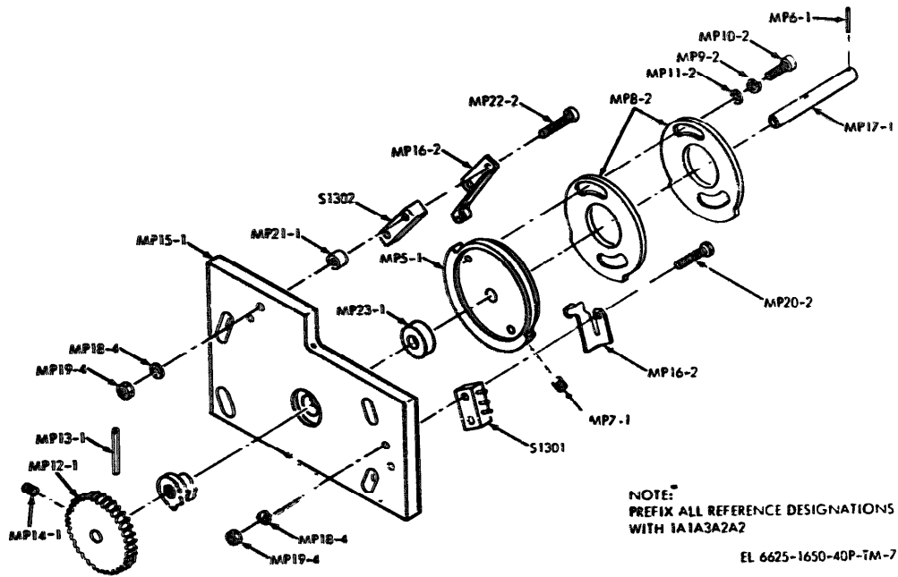
Figure 8. Rear Plate Assembly
