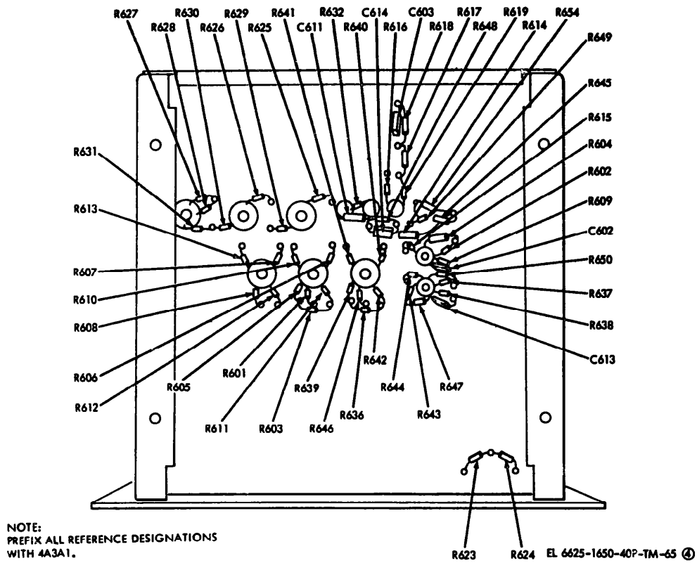
Figure 62. Chassis Assembly (Sheet 4 of 4)
