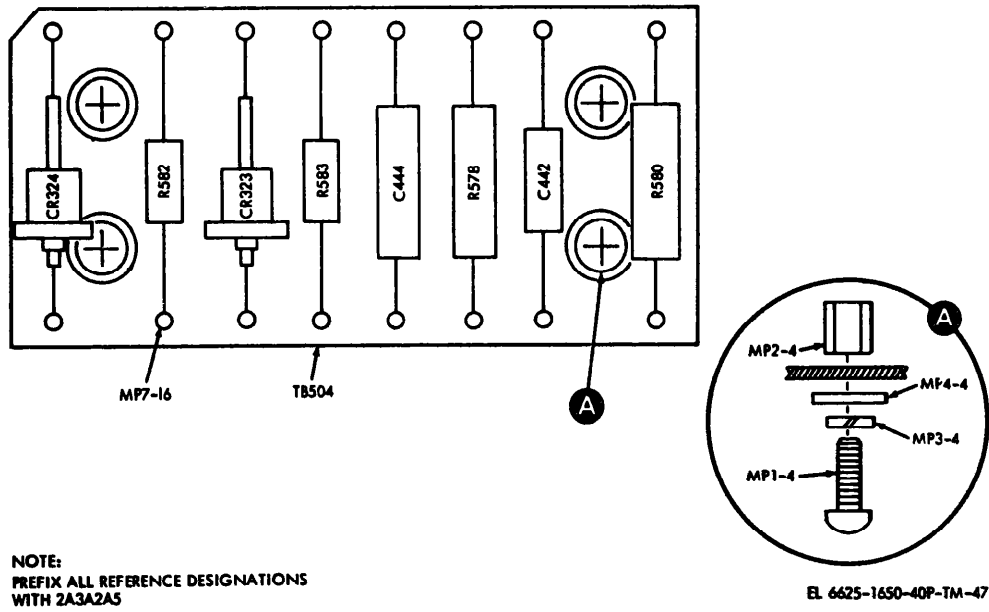
Figure 46. Terminal Board Assembly, 2A3A2A5
