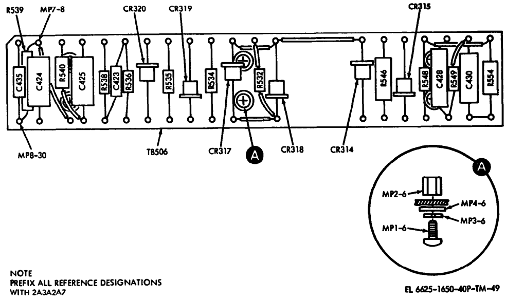
Figure 48. Terminal Board Assembly, 2A3A2A7
