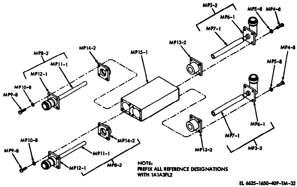
Figure 32. Filter Assembly
