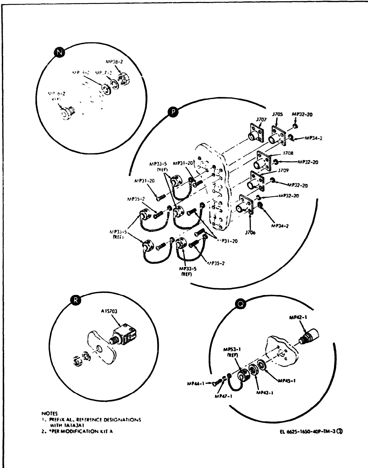
Figure 4. Front Panel Assembly (Sheet 3 of 4)
