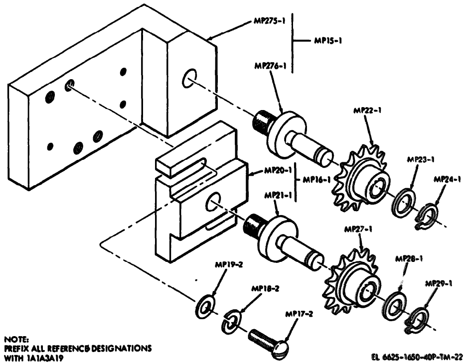
Figure 22. Chain Tightener Assembly
