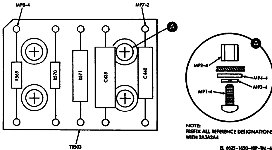
Figure 45. Terminal Board Assembly, 2A3A2A4
