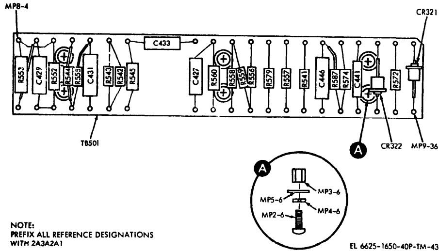
Figure 42. Terminal Board Assembly, 2A3A2A1
